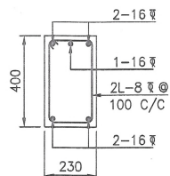
SECTION R-R (SCALE 1:20)
