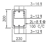
SECTION K-K (SCALE 1:20)
