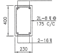
SECTION Z-Z (SCALE 1:20)
