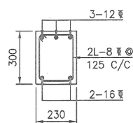
SECTION X-X (SCALE 1:20)
