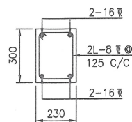
SECTION H-H (SCALE 1:20)
