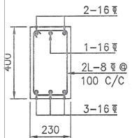
SECTION U-U (SCALE 1:20)
