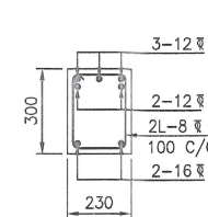
SECTION W-W (SCALE 1:20)
