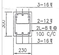
SECTION M-M (SCALE 1:20)
