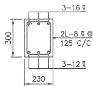
SECTION L-L (SCALE 1:20)
