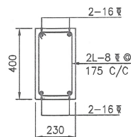
SECTION Q-Q (SCALE 1:20)
