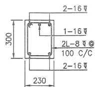
SECTION J-J (SCALE 1:20)
