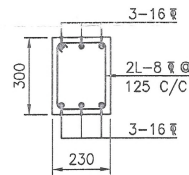
SECTION N-N (SCALE 1:20)
