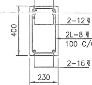
SECTION P-P (SCALE 1:20)
