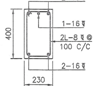
SECTION Y-Y (SCALE 1:20)
